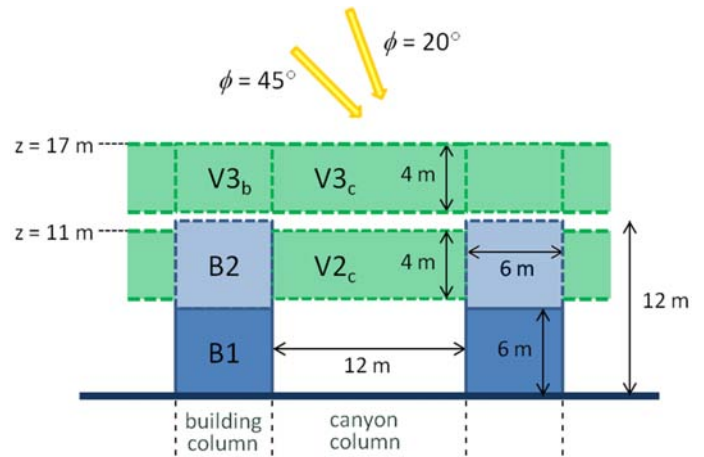
Figure 2. Model geometries and solar zenith angles for shortwave radiation system response tests. “B” = building, “V” = vegetation foliage, numbers refer to vertical layer, and subscripts refer to building (e.g. “V3 b ”) or canyon (e.g. “V3 c ”) columns. Vertical resolution is 1 m and solar azimuth is perpendicular to the canyon orientation for all simulations.
