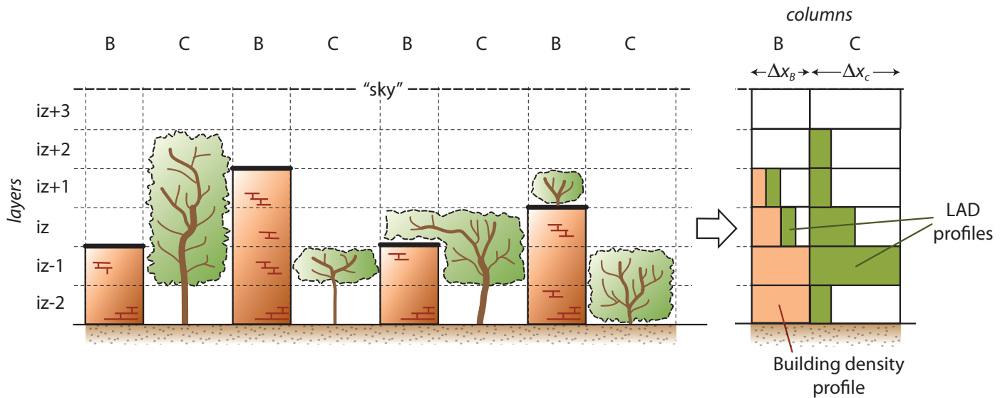
Figure 1. A two-dimensional view of the conceptualization of the urban surface that underlies the model geometry: equal width and equally-spaced buildings with a height frequency distribution, randomly ordered in the horizontal. Foliage layers of different densities are present above and between buildings and at random horizontal locations. An example urban height distribution, building order, and foliage distribution is shown. B = building column; C = canyon column.
