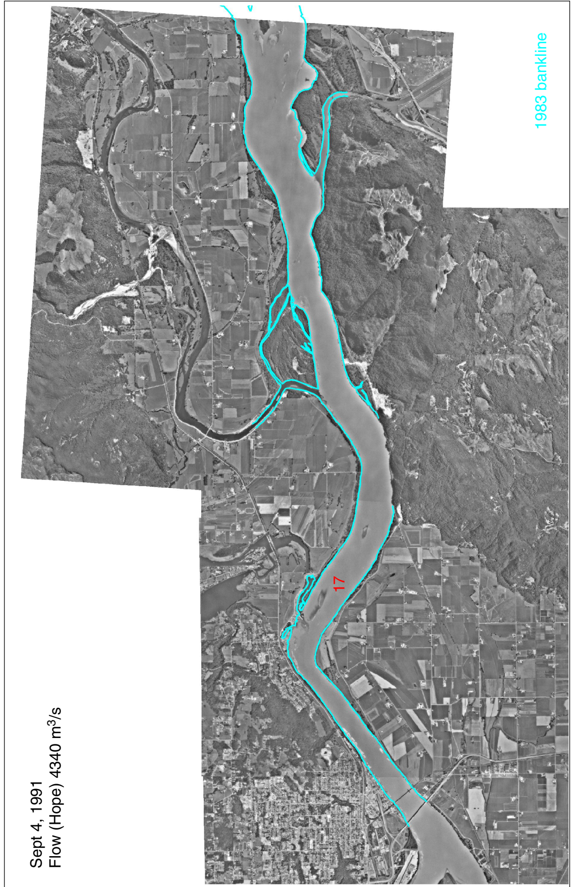
Figure C-17. Vedder River to Mission railway bridge reach, 1991 - 1999.
