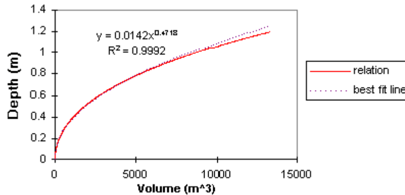
Figure 5-7 Depth-volume relation
