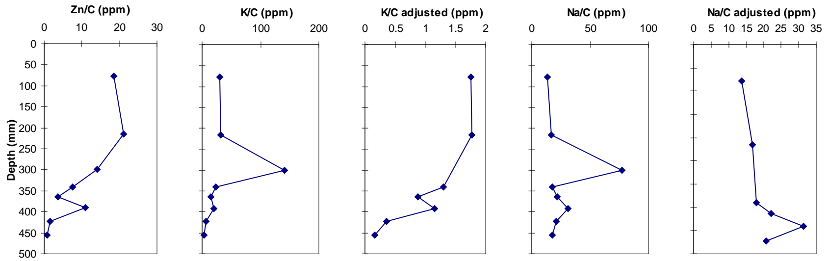
Figure 6-15 AL4 heavy metal profiles normalized for carbon
