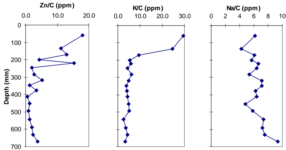
Figure 6-16 BL1 metal profiles normalized for carbon
