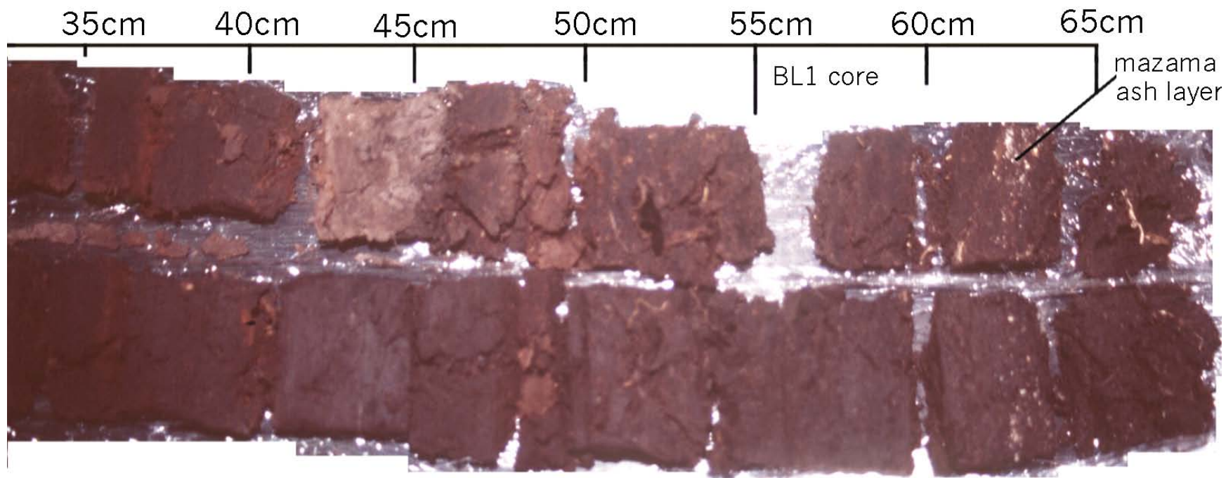
Figure 6-7 Bottom section of the BL1 core
