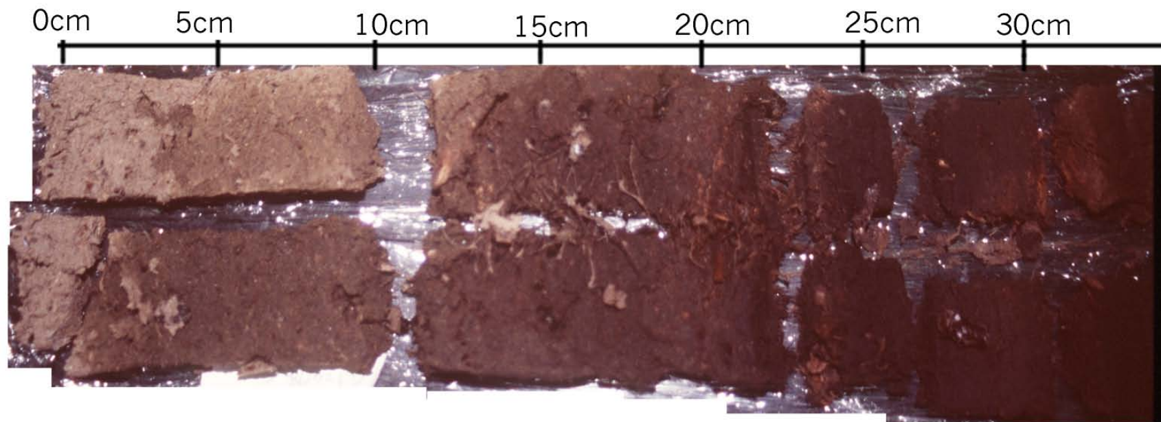
Figure 6-5 Top section of the BL1 core
