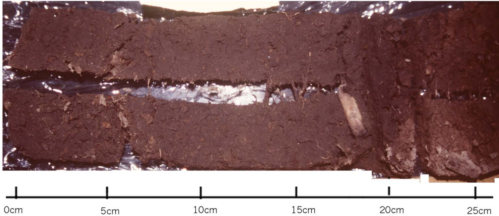
Figure 6-8 Top section of the AL3 core
