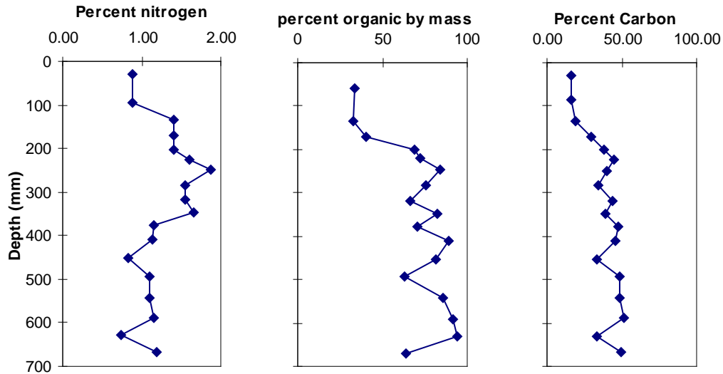
Figure 6-12 Nitrogen, carbon, organic, and C:N ratio profiles
