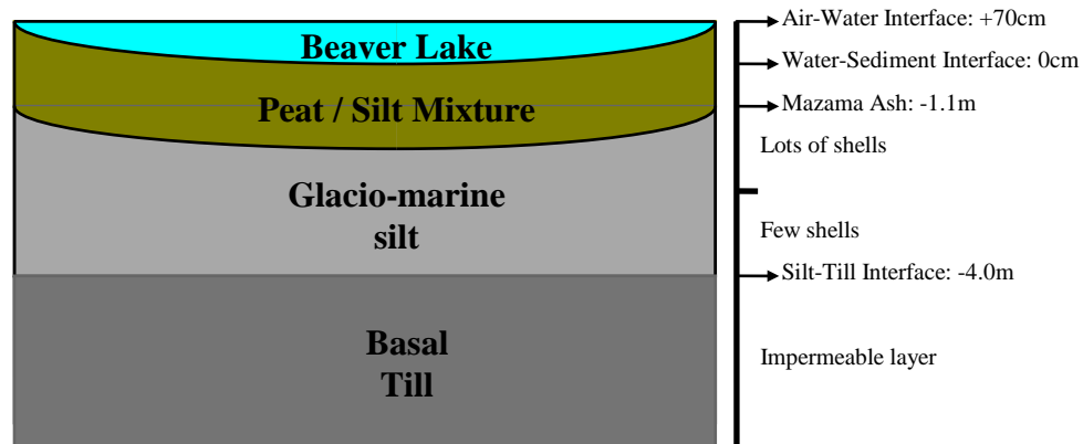
Figure 6-3 schematic sediment profile of the lake
